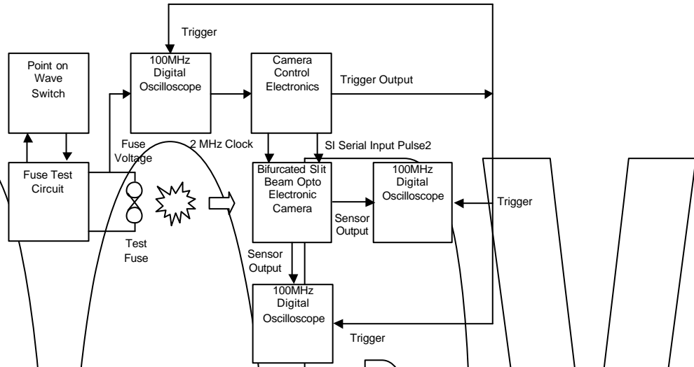
Fig. 2. Schematic diagram of opto-electronic camera control, optical system and fuse test circuit.
