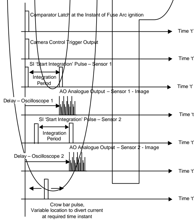
Figure 3 Diagram indicating control pulse (SI) and camera image (AO) capture instances
