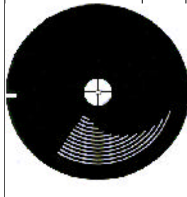
Fig. 6i Patterned-encoded wheel, typical of sequential arc ignition
