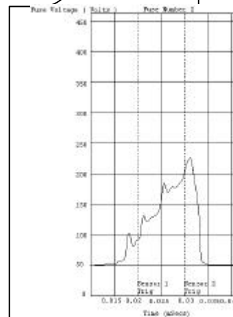
Fig. 7ii Fuse voltage oscillogram – with current 'crow-barred' 5 \mu s after Sensor 2 triggered
